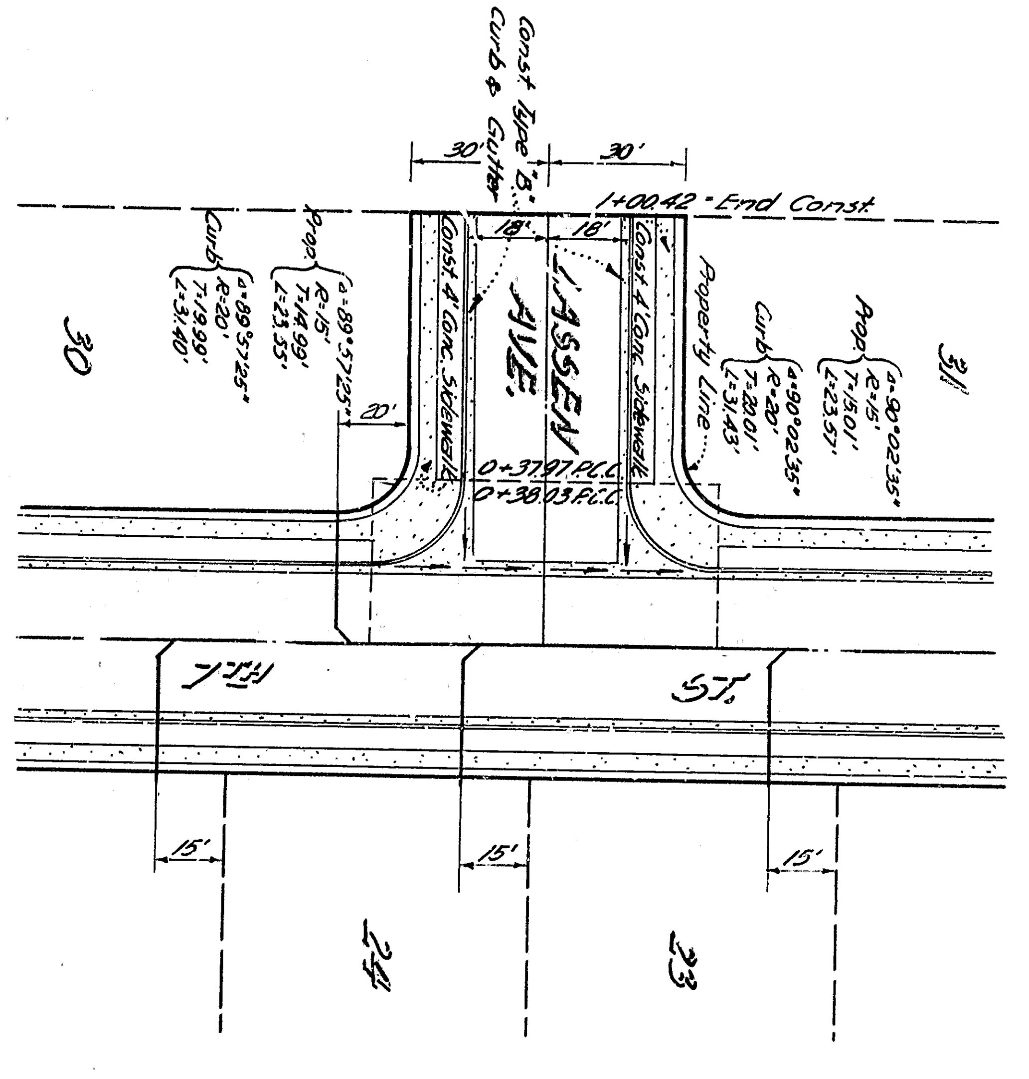
PLAN LASSEN AVENUE Scale 1"=40'
