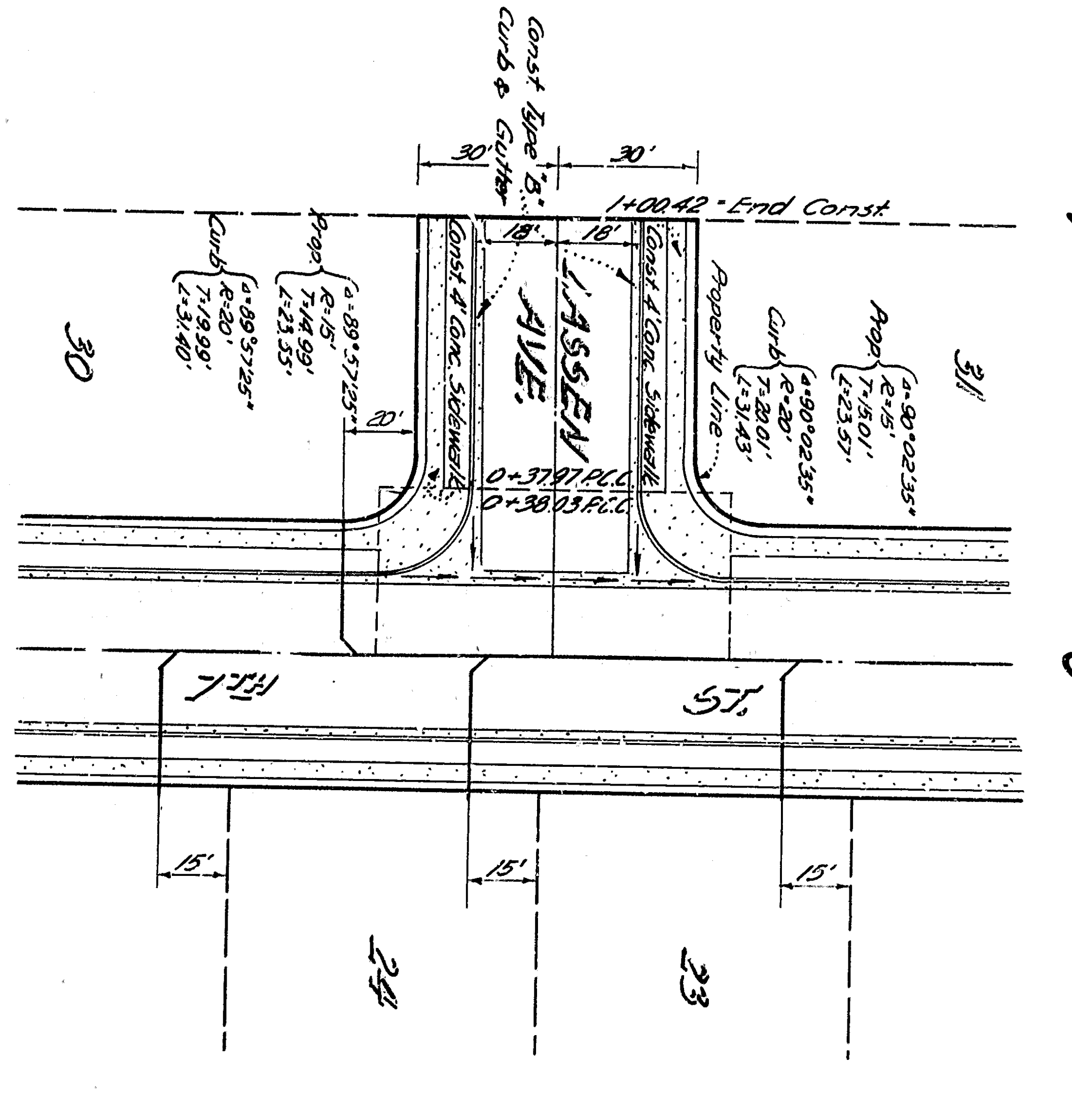
PLAN LASSEN AVENUE Scale 1"=40'
