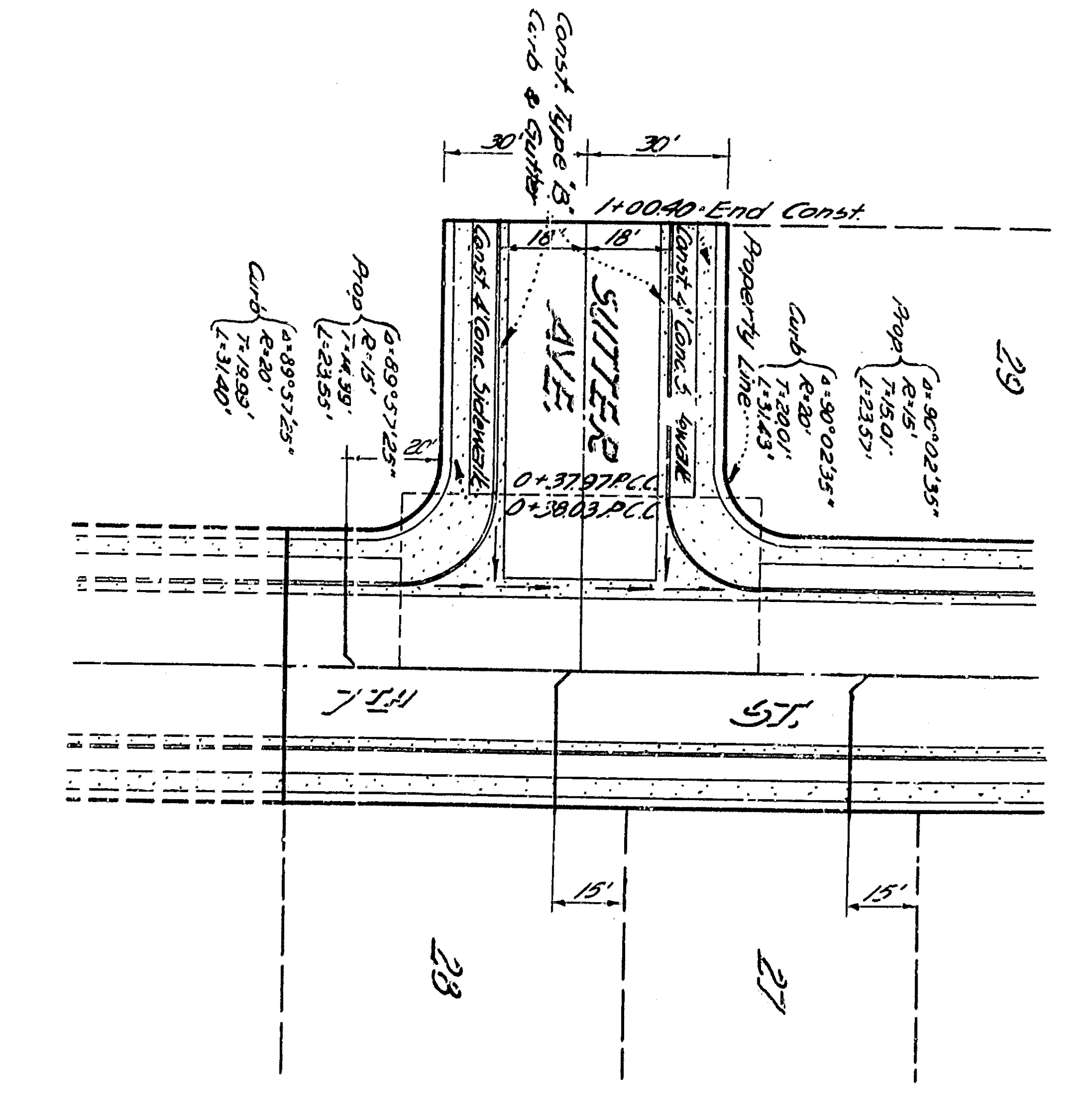
PLAN SUTTER AVENUE Scale 1"=40'
