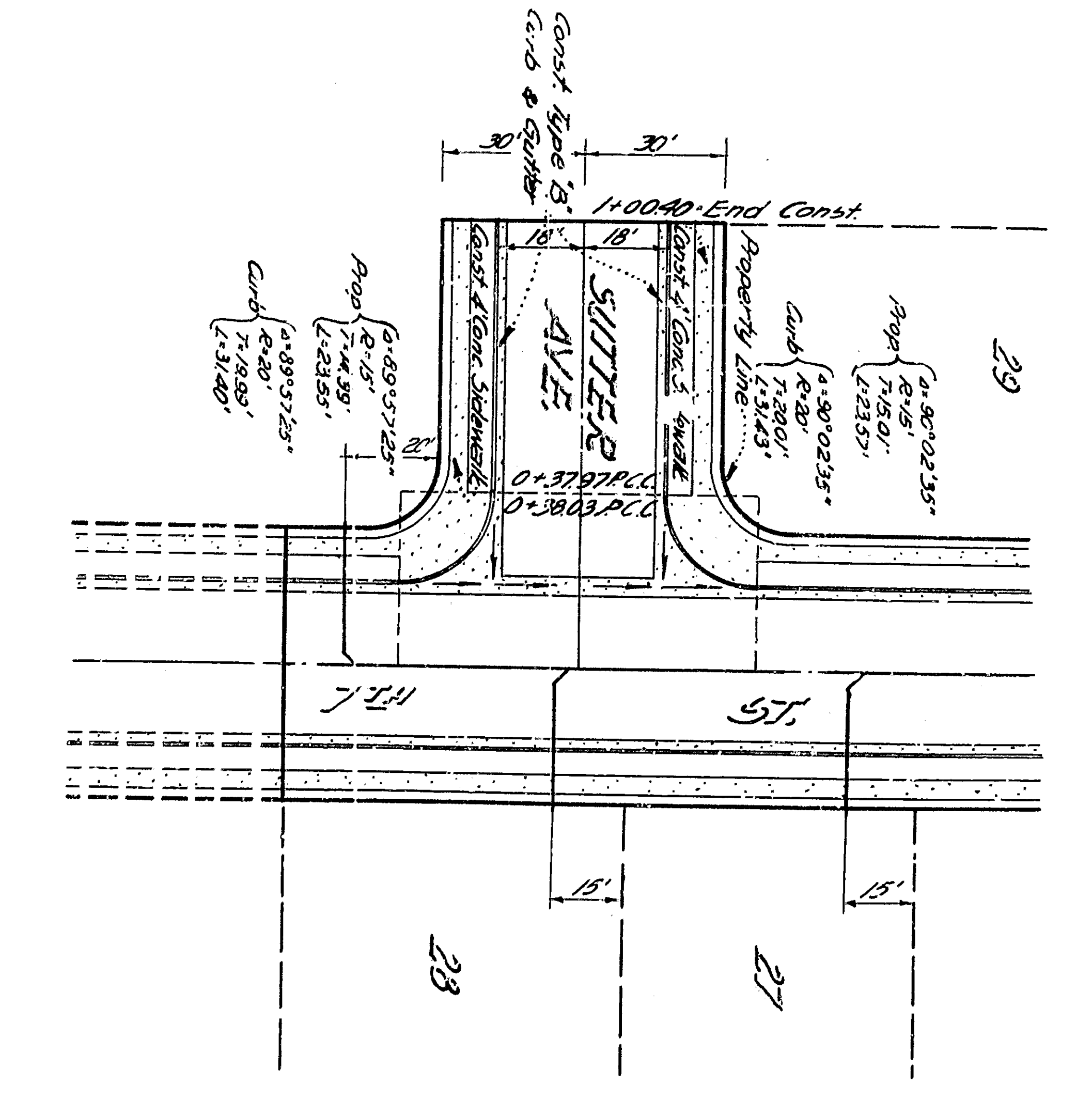
PLAN SUTTER AVENUE Scale 1"=40'
